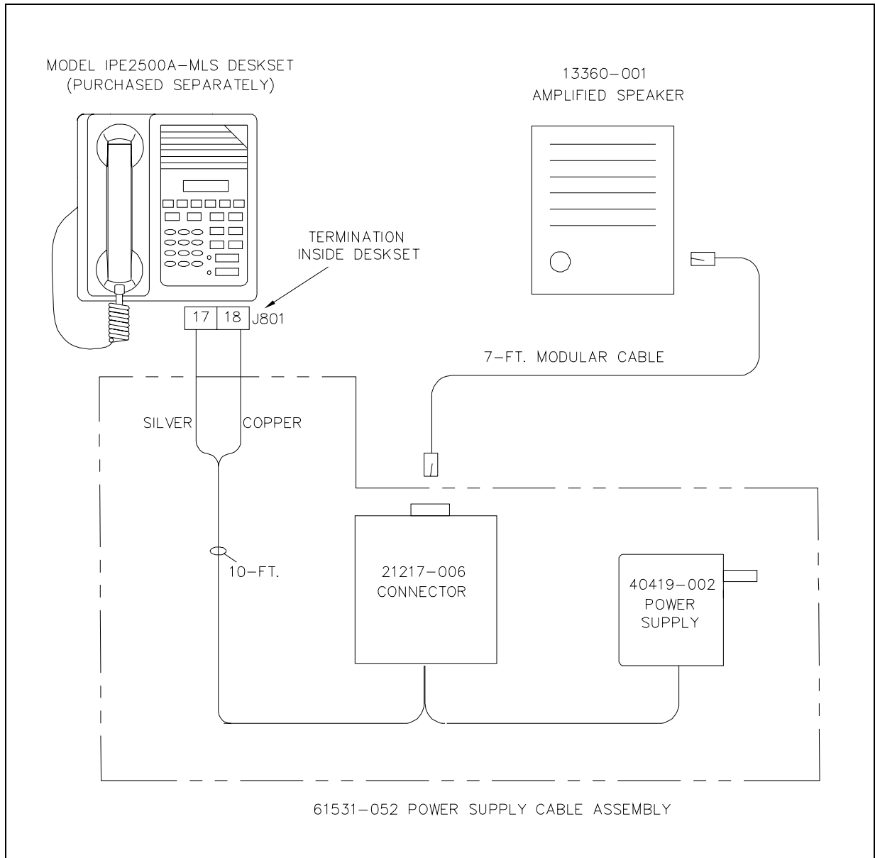
Figure 1. Model XAC0120A External Speaker Connections
